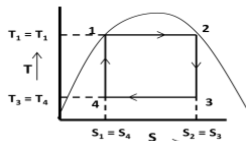
(T-s diagram)
